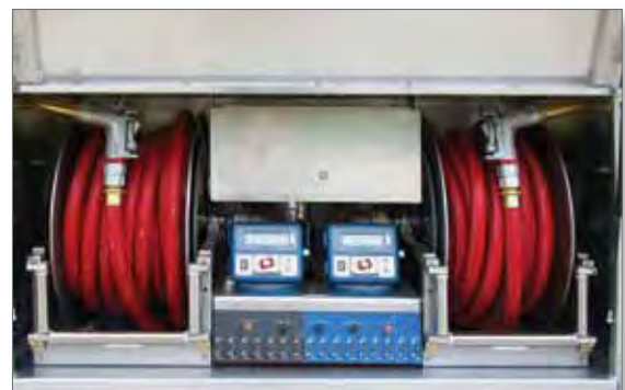
Dual Systems Remotely Mounted LCR II Registers
